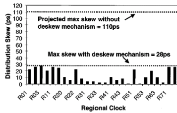
Fig. 10. Experimental skew measurements.
