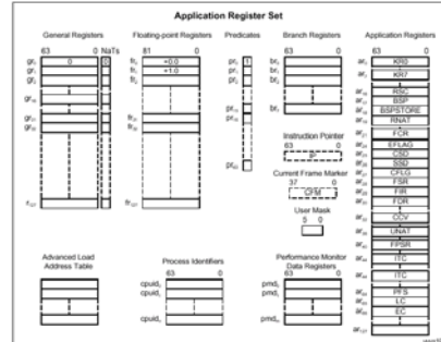
Figure 3-1. Application Register Model
