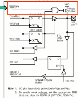
FIGURE 3-3: BLOCK DIAGRAM OF RB3:RB0 PINS
